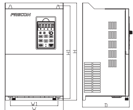
5.5-110kW structure diagram
