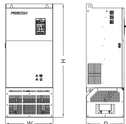
132-200kW structure diagram
