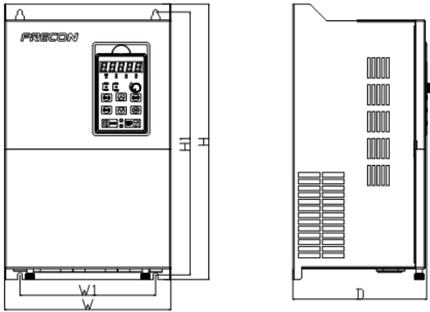
Fig 1-3 5.5 ~ 110kW Wall installation diagram
